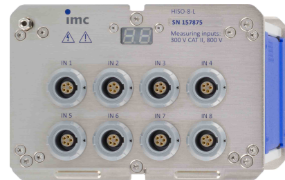
CRFX/HISO-8-L
