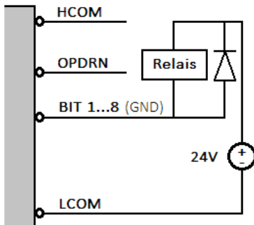
Open Drain
